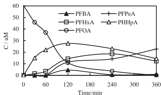
Figure 4. Changes in the concentrations of PFOA and intermediates.
