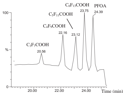
Figure 3. TIC spectra of PFOA and its decomposition products.
