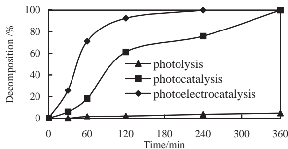
Figure 1. Decomposition of PFOA with reaction time.
