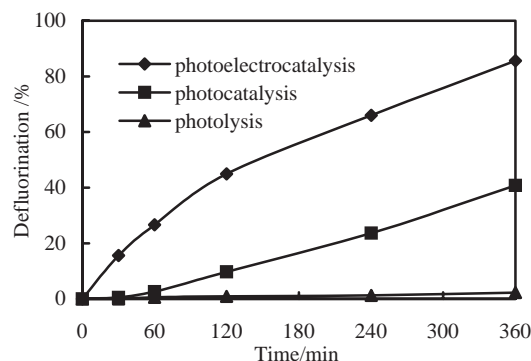
Figure 2. Defluorination of PFOA with reaction time.
